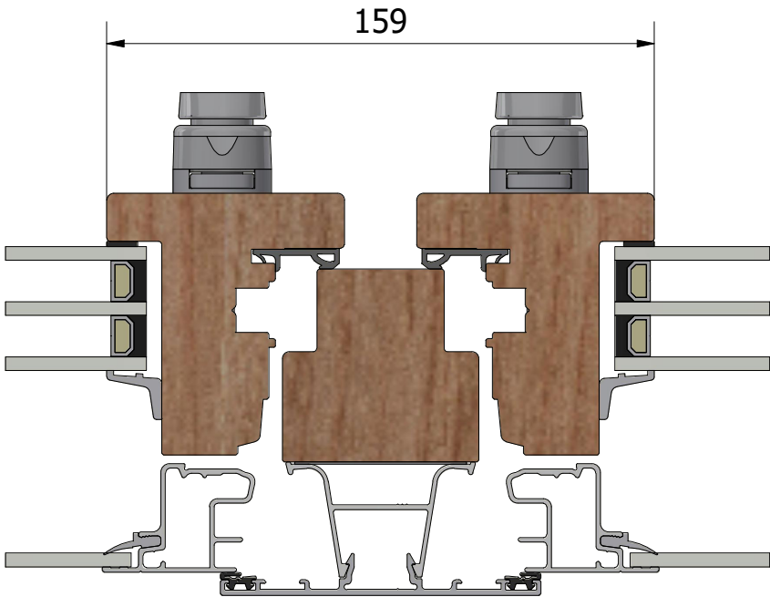
Karmpost
